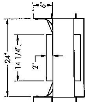
SECTION A-A SCALE 2X
